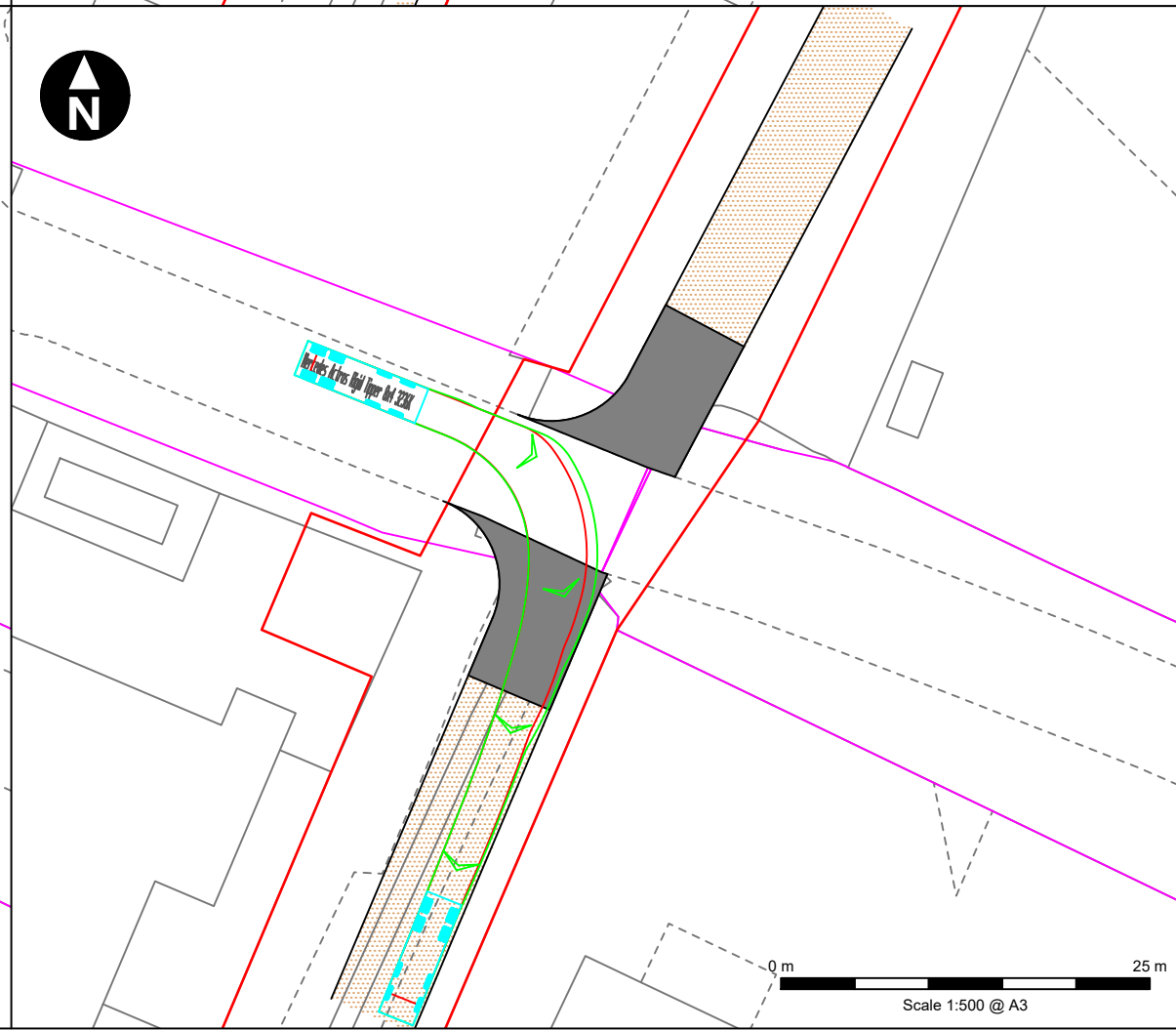
Figure 10.3ii Proposed Construction Access Weasenham Lane SPA
