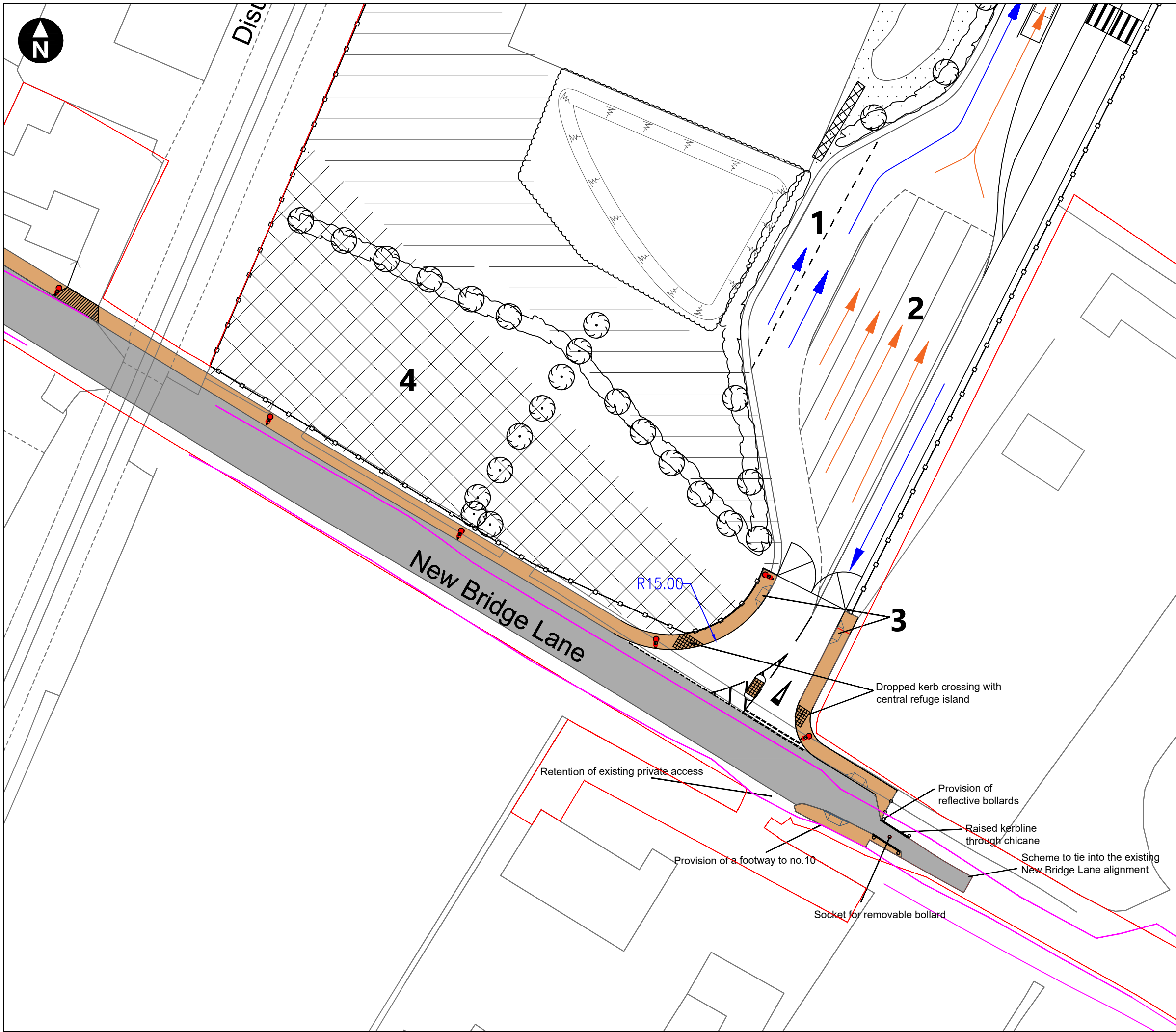
Figure 10.1i New Bridge Lane access design
