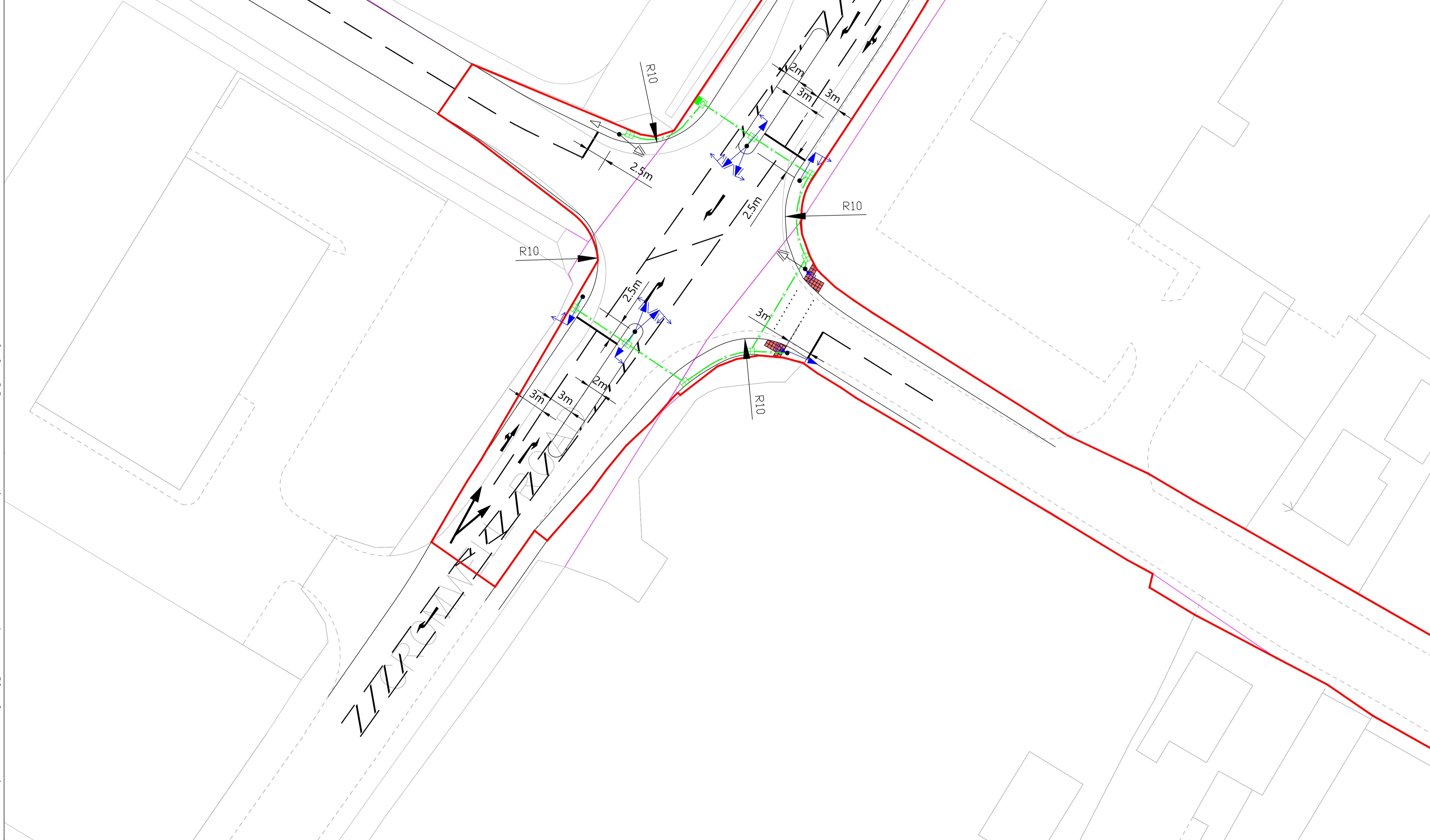
Figure 10.1iv Cromwell Road/New Bridge Lane Signal Scheme - General arrangement with indicative ducting
